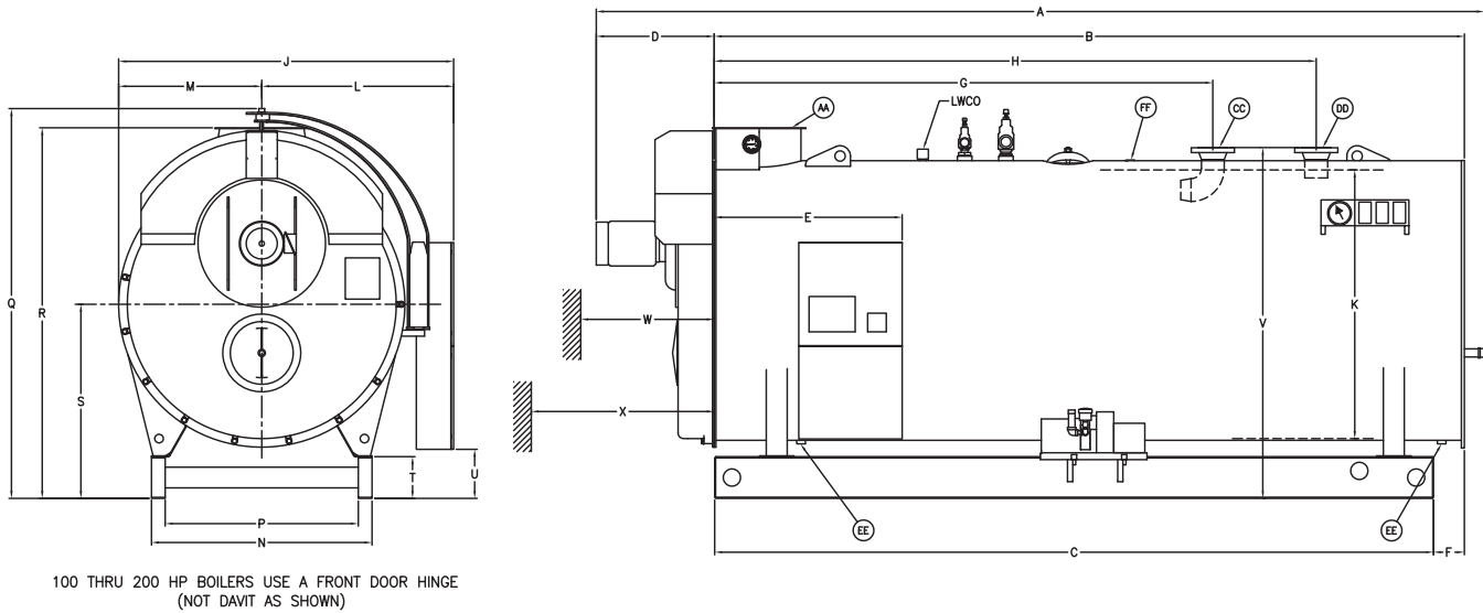
Figure 2. CBEX-2W Hot Water Boiler Dimensions, 100-800 HP
