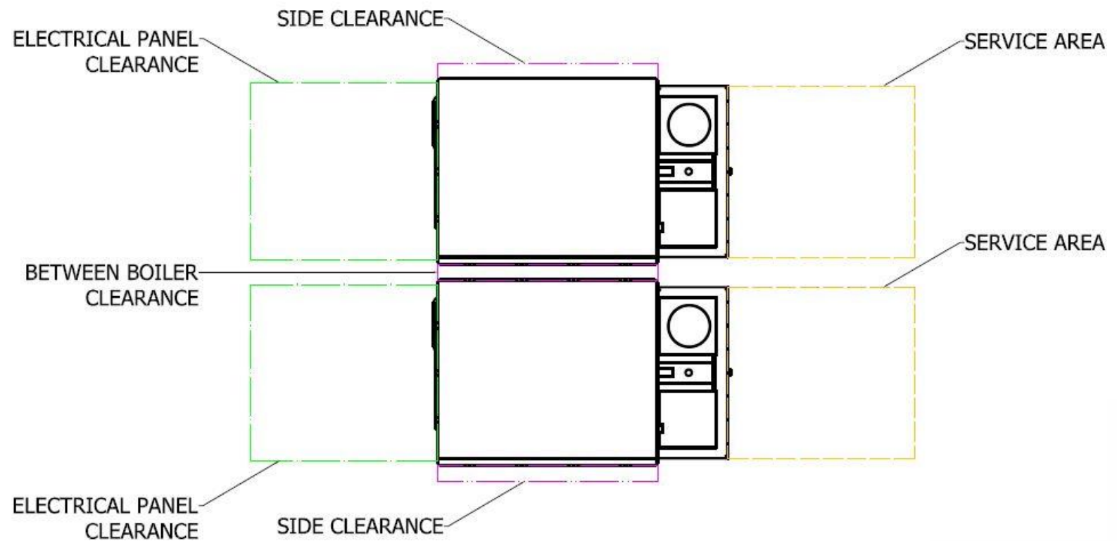
TOP VIEW
